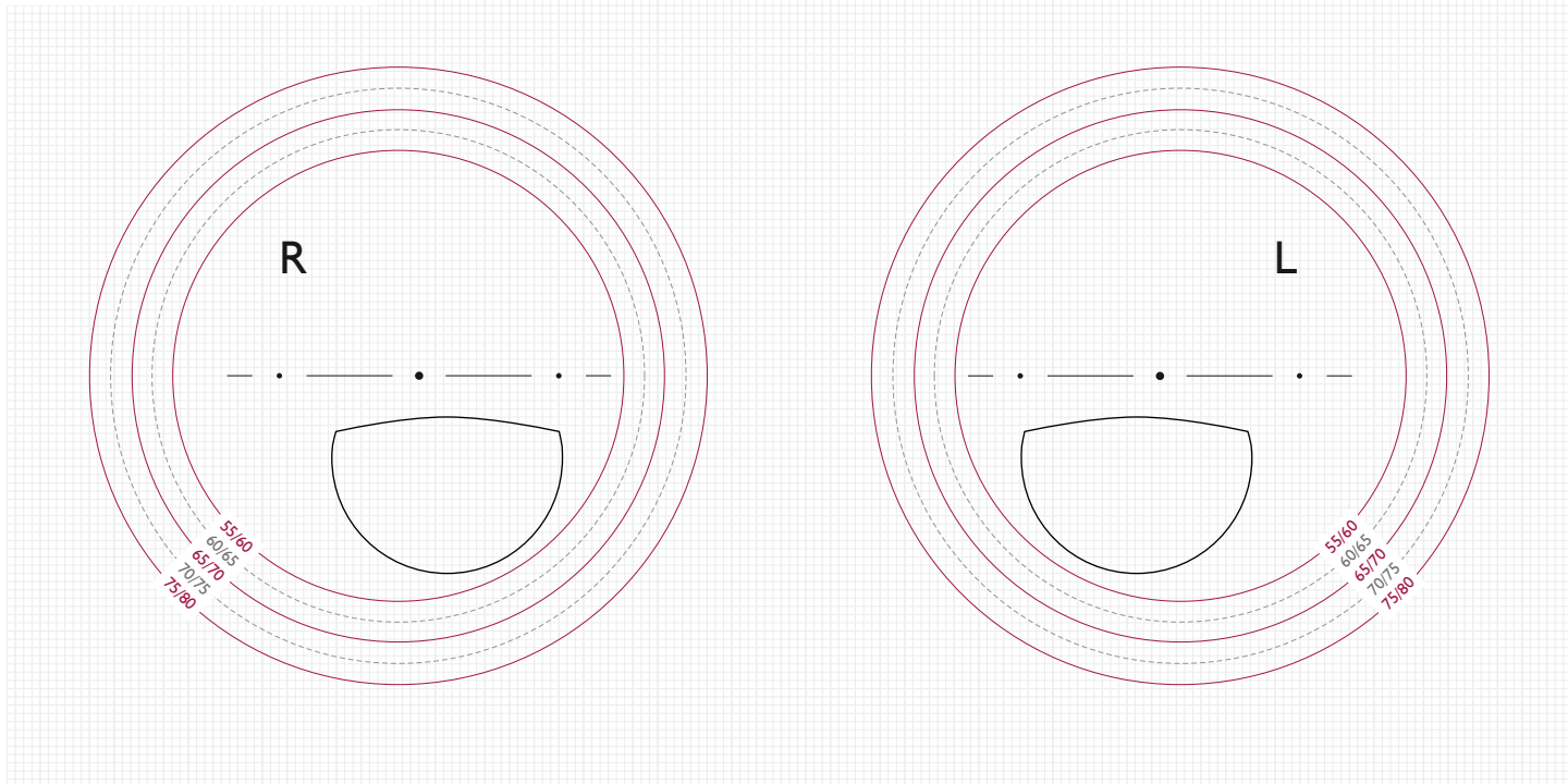
BI-FOCAL C28 (ind. 1.50/1.61)
